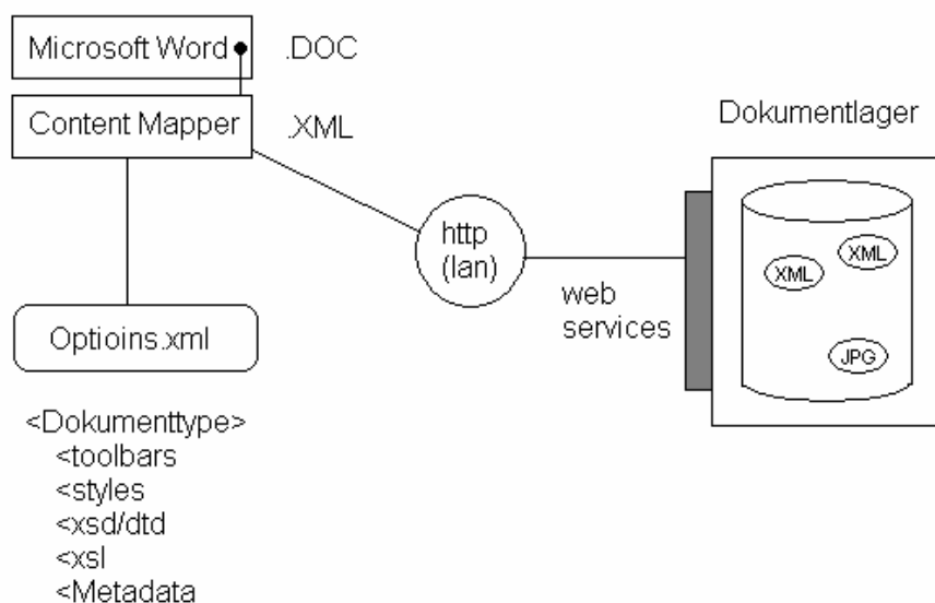
Figur 9.4: Kart over Content Mapper
